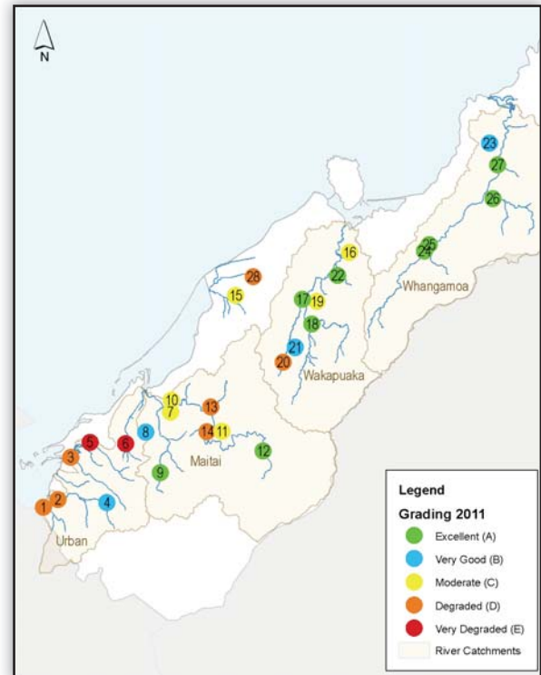
Fig. 1. Nelson river and stream water quality grades, 2011.
